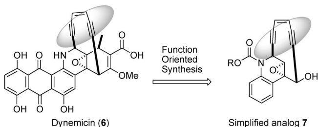
FIGURE 5. Dynemicin and a simplified functional analog.
